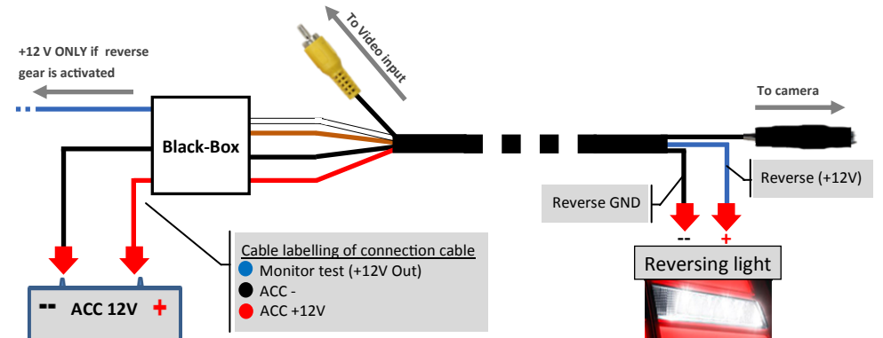
Exchange rear door opener handle with integrated camera (exemplifying figure)
