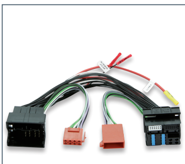
AP T-Harness ("AP T-H AVS01" in the picture)
